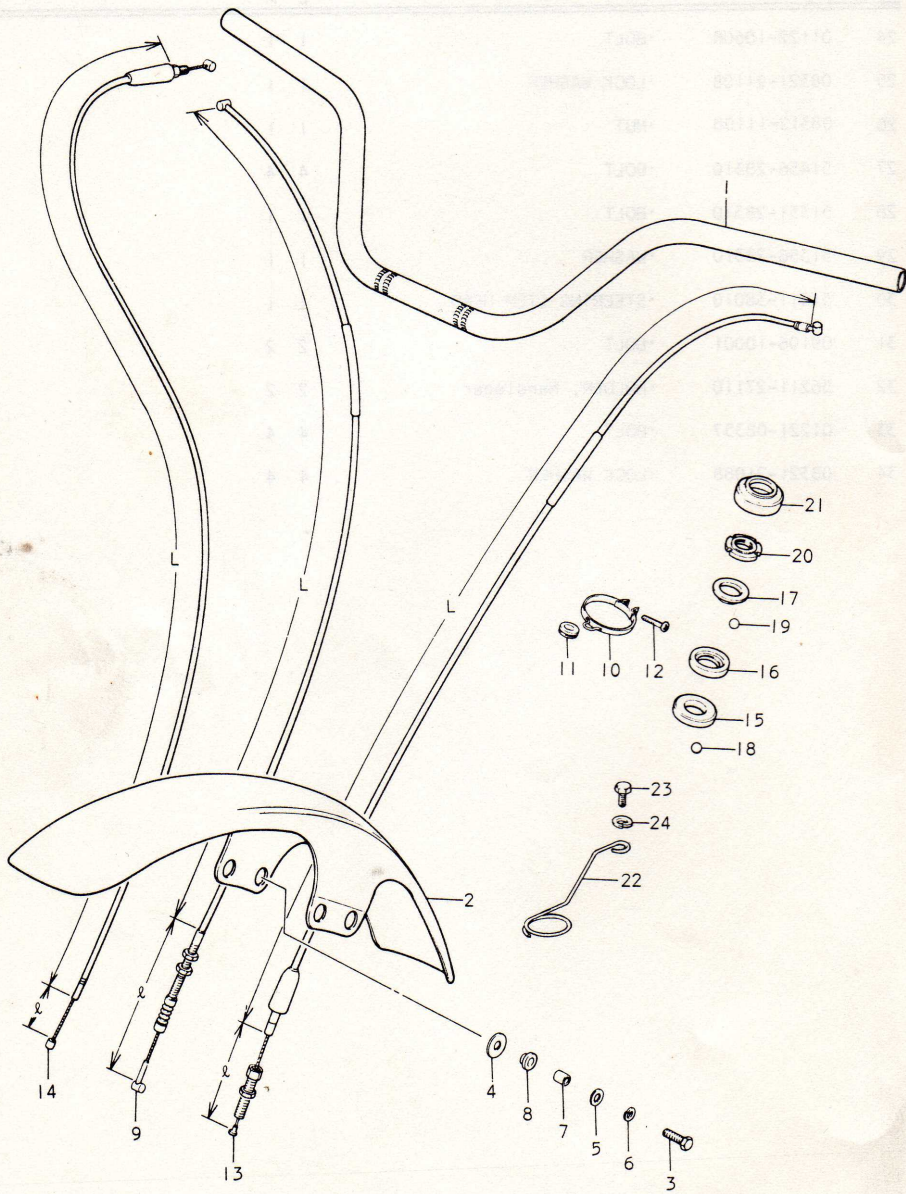
FIG.17 HANDLEBAR - FRONT FENDER
