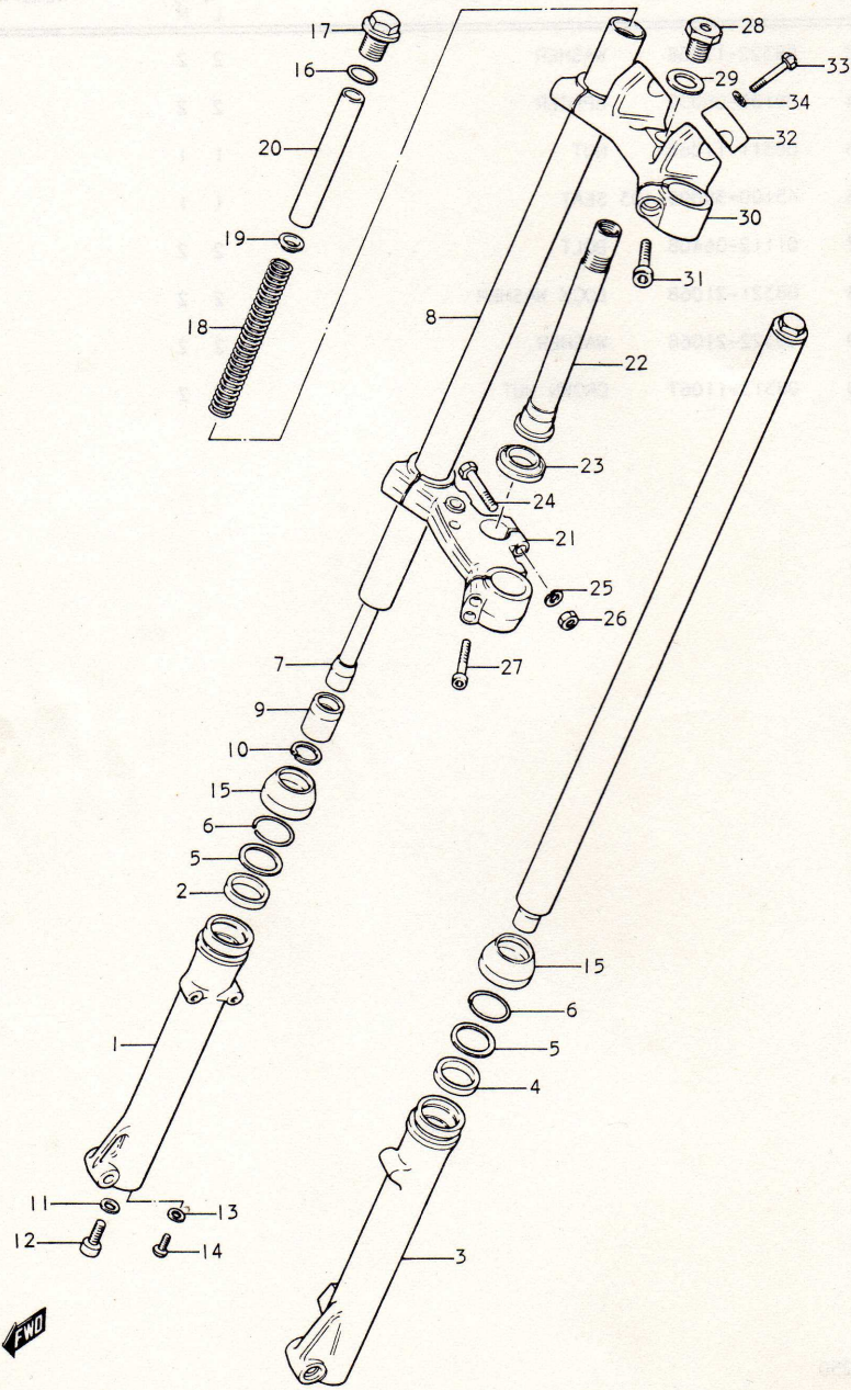
TA32 FIG.16 FRONT FORK
