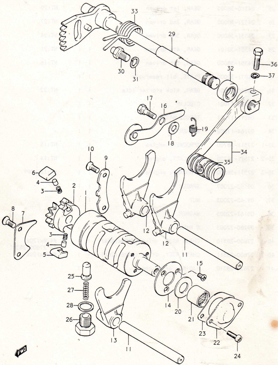
FIG.9 GEAR SHIFTING
